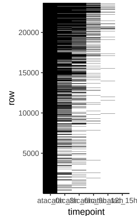
Oct4-Sox2
