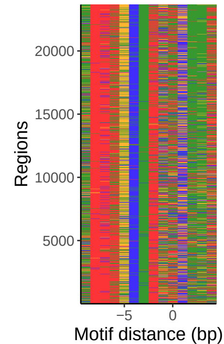
Oct4-Sox2
