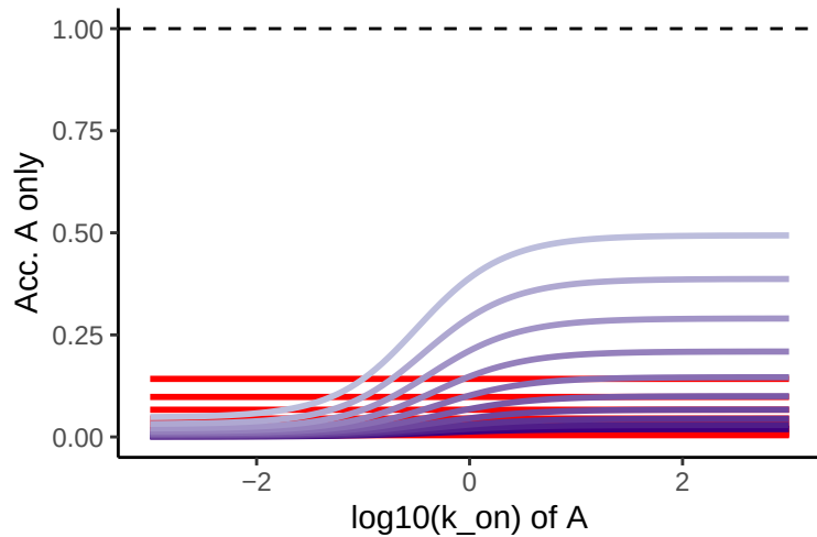
Sox2 on Sox2 motif k_close
