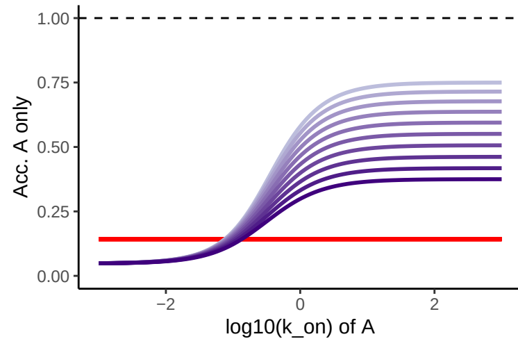
Sox2 on Sox2 motif closing
