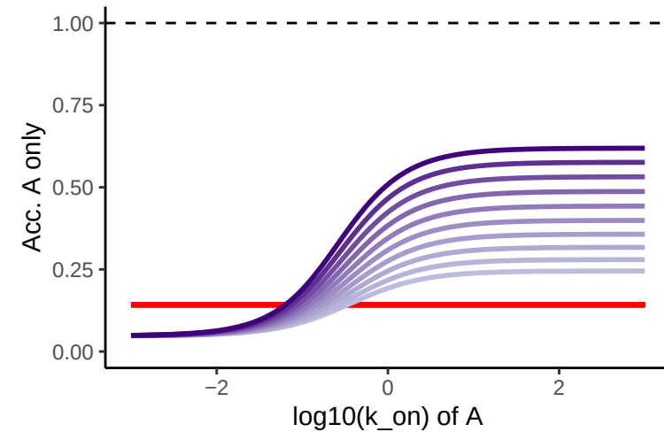
Sox2 on Sox2 motif opening
