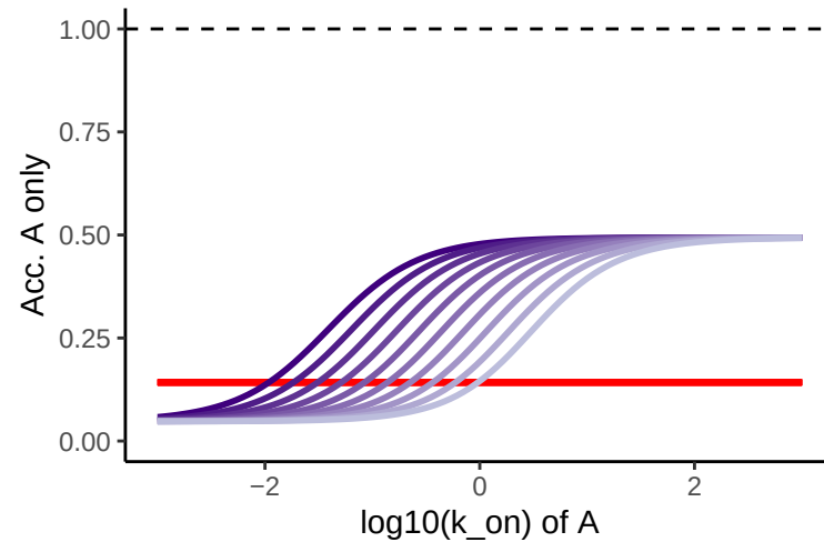
Sox2 on Sox2 motif affinity
