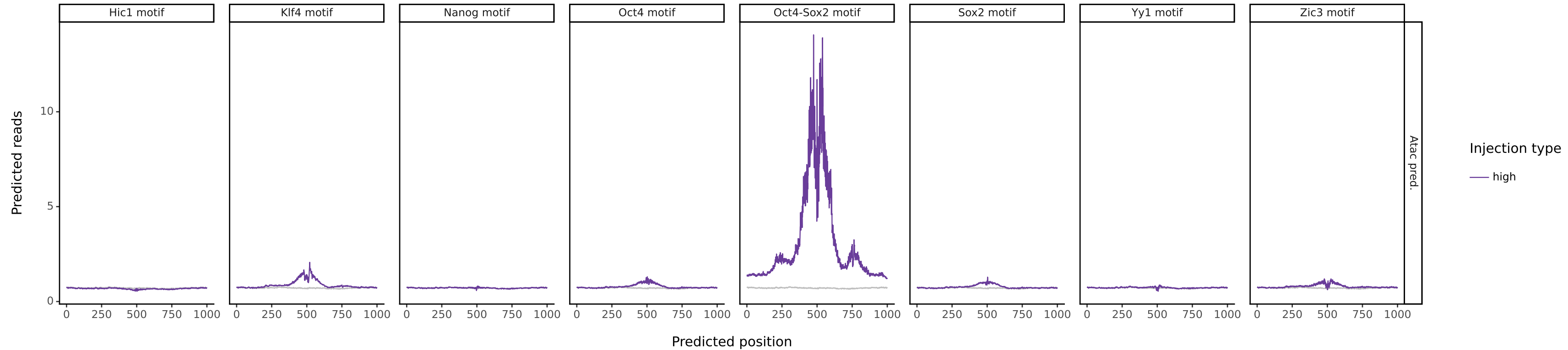
atac_wt_across_genome
