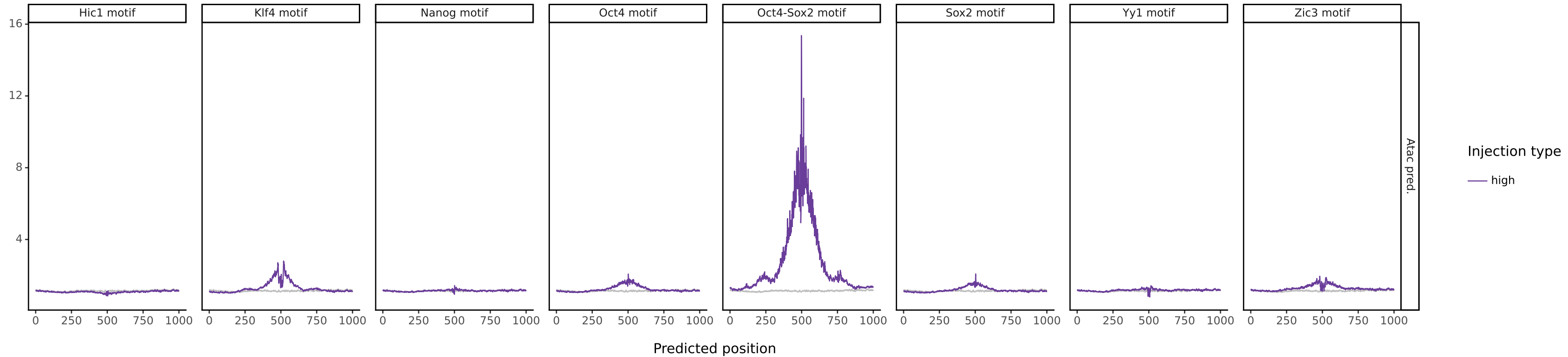
atac_wt_across_split
