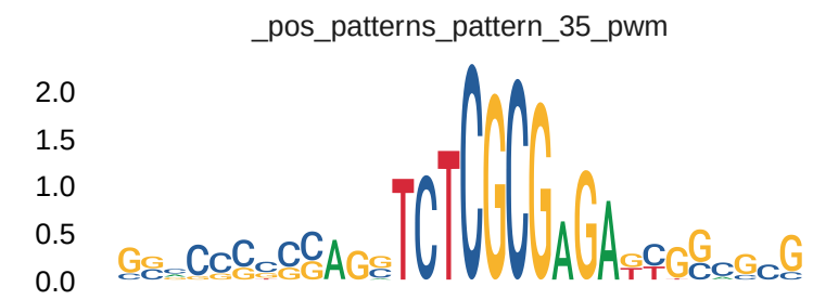
fold2_atac_wt
