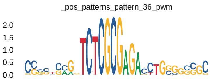
fold1_atac_wt
