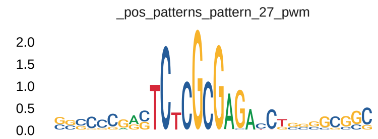
fold3_atac_wt
