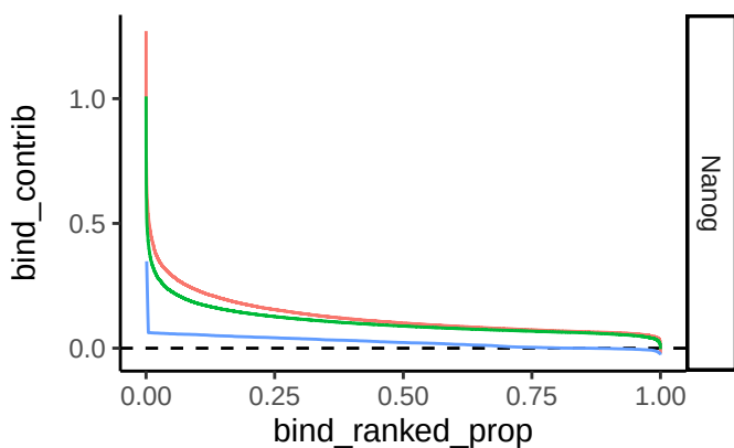
rank_type
