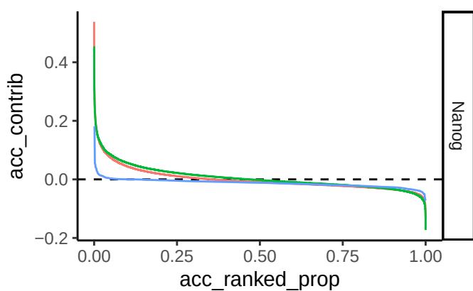
rank_type
