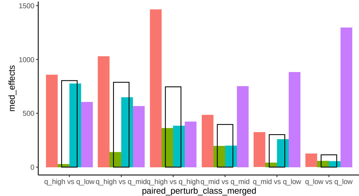
pred levels
