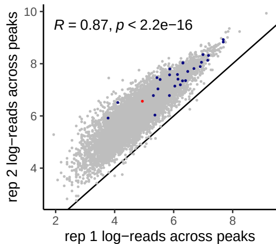
mesc_Akr1cl_scenario_context_mut_nBsox2krlxuscna_positiocontext_mut_nBsox2krlxuscna_positiocontext
