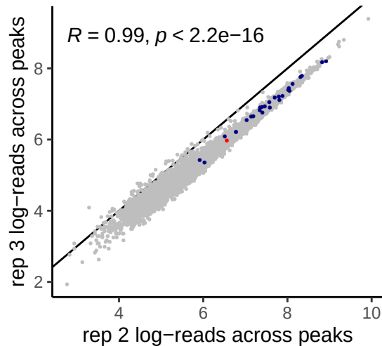
mesc_Akr1cl_scenario_context_mut_nBsox2krlxuscna_positiocontext_mut_nBsox2krlxuscna_positiocontext
