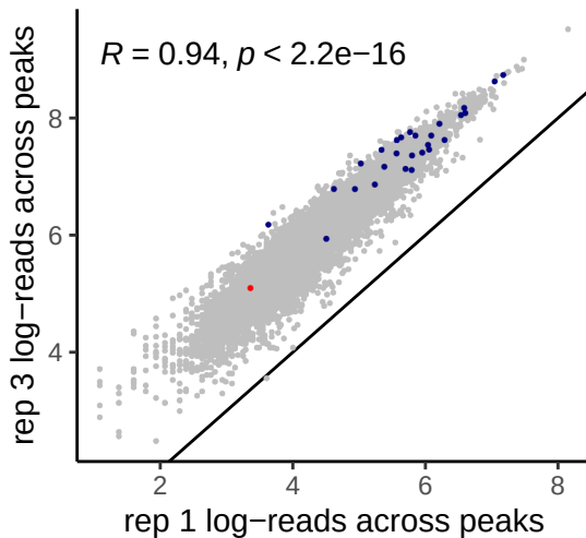
mesc_Akr1cl_scenario_context_mut_nBsox2krlxuscna_positiocontext_mut_nBsox2krlxuscna_positiocontext
