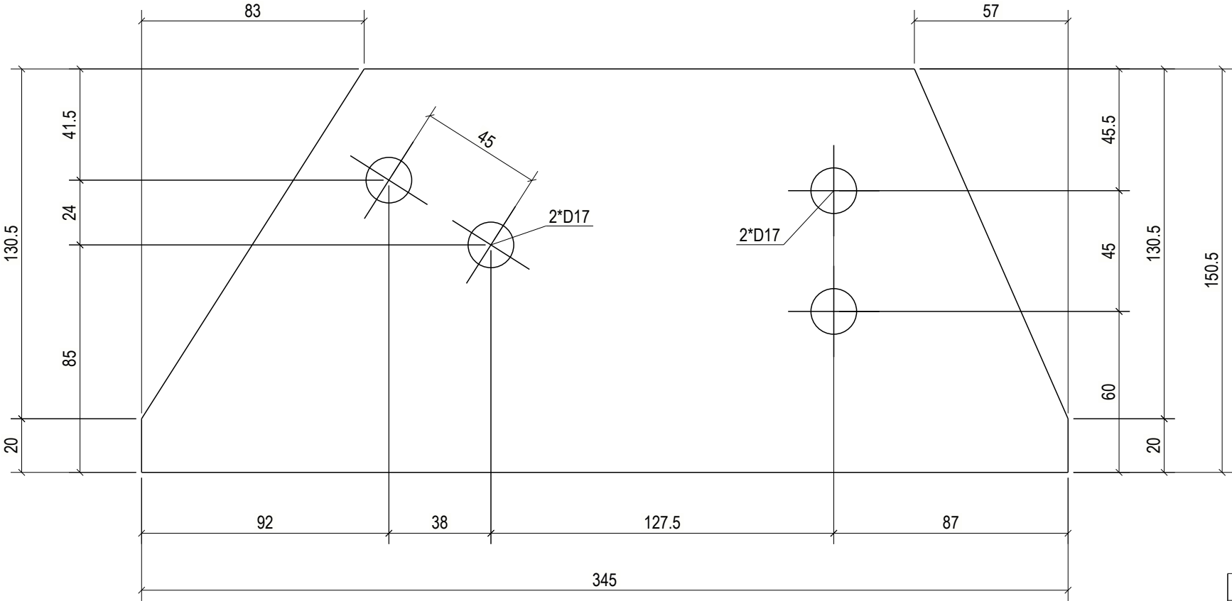
FRONT VIEW
