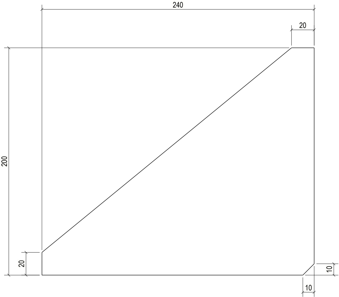
FRONT VIEW
