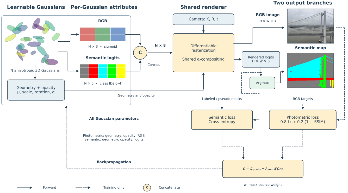
Figure 4. Semantic Gaussian representation and joint rendering. Each Gaussian carries geometry, opacity, RGB, and five semantic logits. Concatenated RGB and logits are rendered with shared alpha-compositing weights. Rendered logits feed cross-entropy during training and argmax for class-map generation. Photometric loss supervises RGB; both losses update shared geometry and opacity. Dashed arrows denote training connections. Semantic colors illustrate class IDs.
