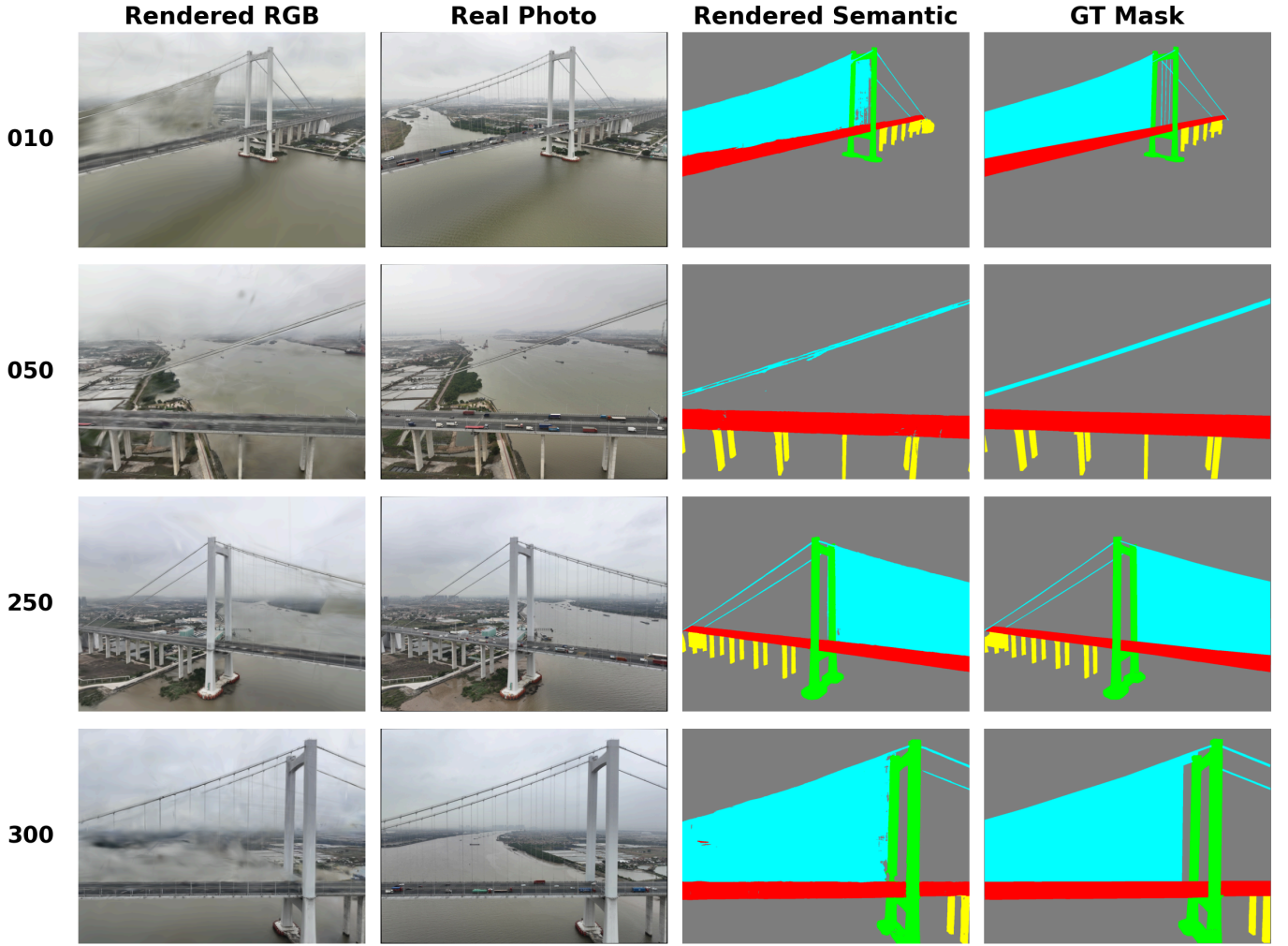
Figure 6. RGB and semantic renders vs. ground truth on four held-out views (010, 050, 250, 300): rendered RGB, real photograph, rendered semantic map, and ground-truth mask. Only the two semantic columns use the class-color palette; RGB columns retain image colors.
