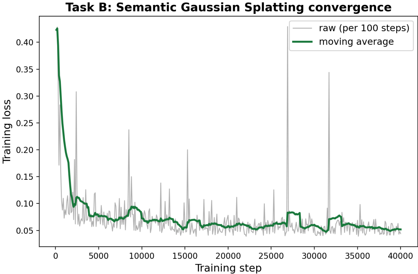
Figure 10. Task B loss for the full-resolution 40,000-step run: single-view samples logged every 100 steps (gray) and their 15-sample trailing moving average (green). These are training losses, not test metrics.
