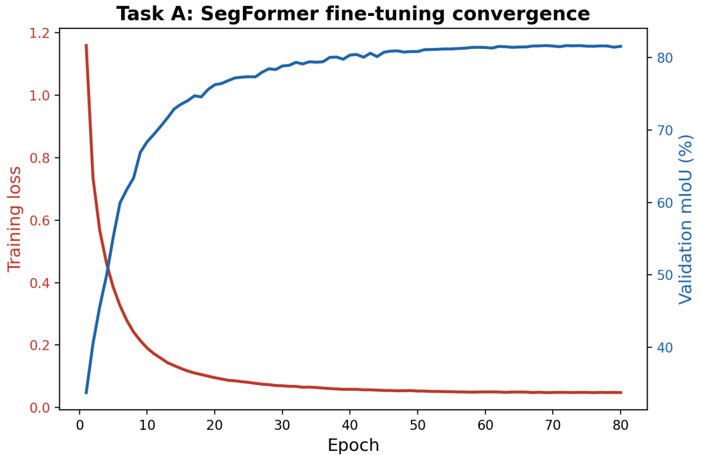
Figure 9. Task A training loss (red, left axis) and structural validation mIoU (blue, right axis) over 80 epochs. Training uses 240 images; validation uses the separate 30-image internal split. The final 30-image test set is not used for checkpoint selection.
