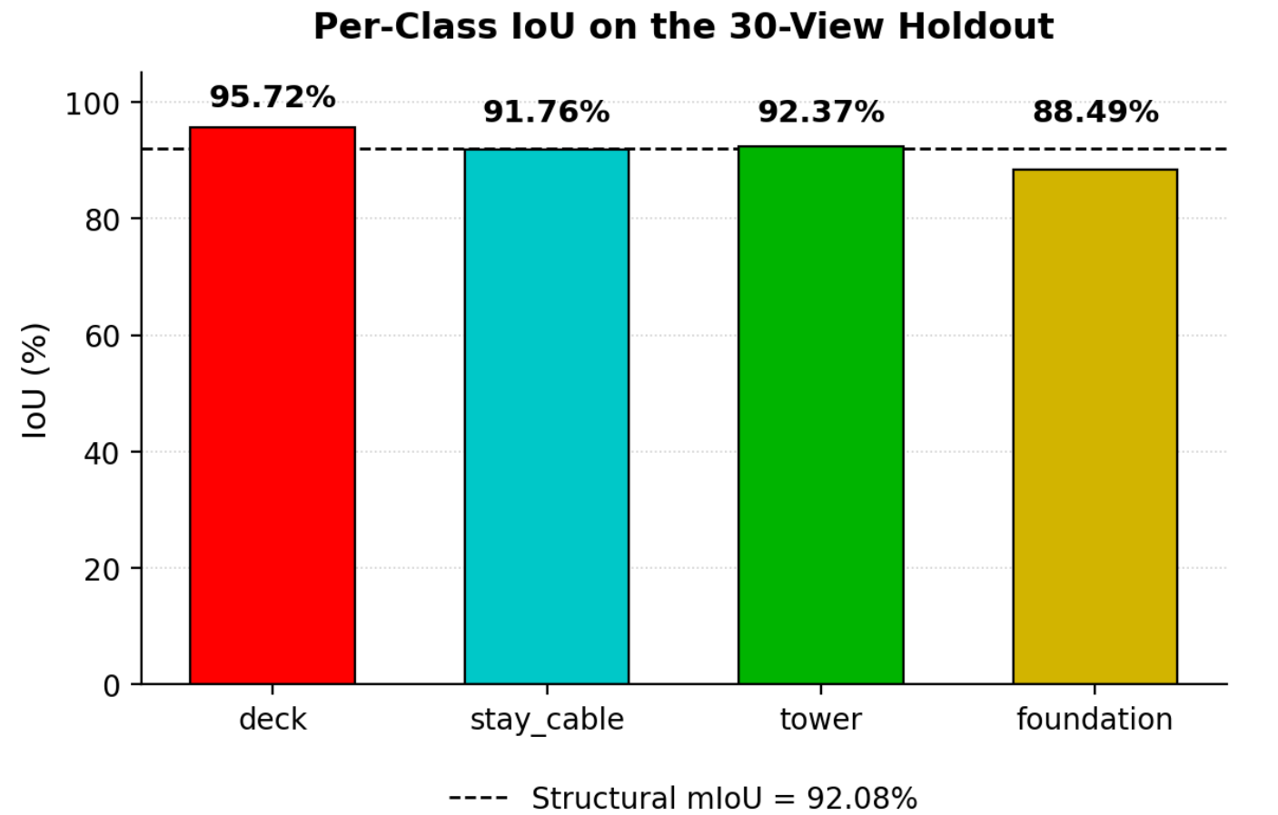
Figure 5. Structural-class IoUs on 30 test views. Class colors identify components; the dashed line marks structural mIoU (92.08%). The vertical axis starts at zero. Background IoU is reported separately in Table 3.
