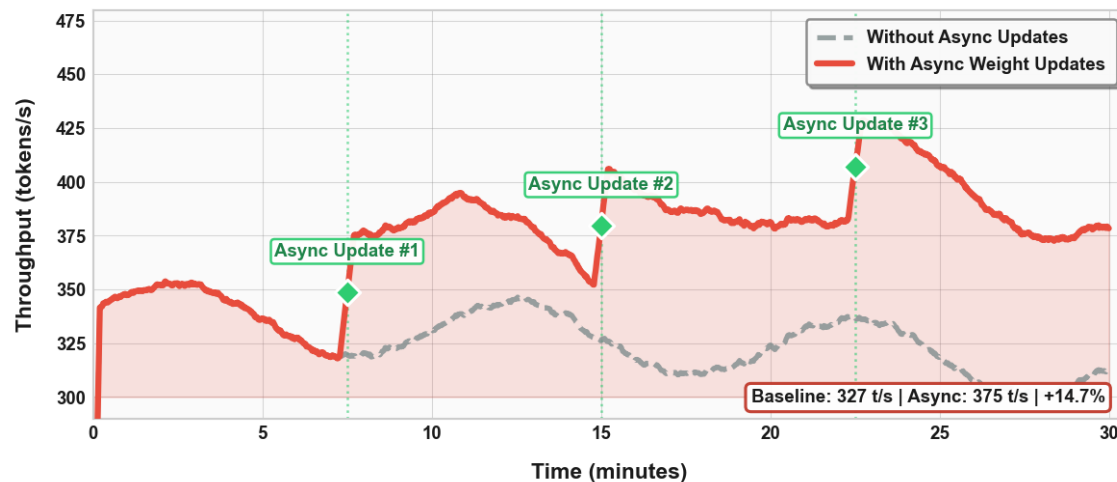
Throughput Over Time with Async Weight Updates
