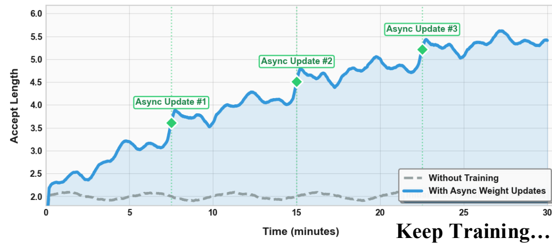
Accept Length Over Time with Async Weight Updates
