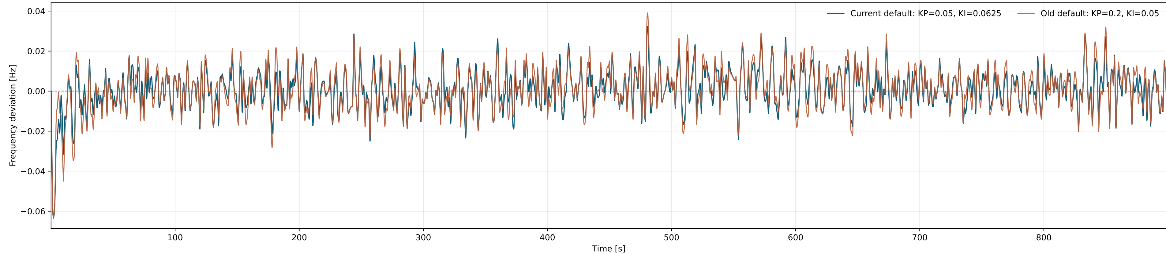
H13D2 Frequency Deviation Comparison (AGC interval = 4 s, wide view)
