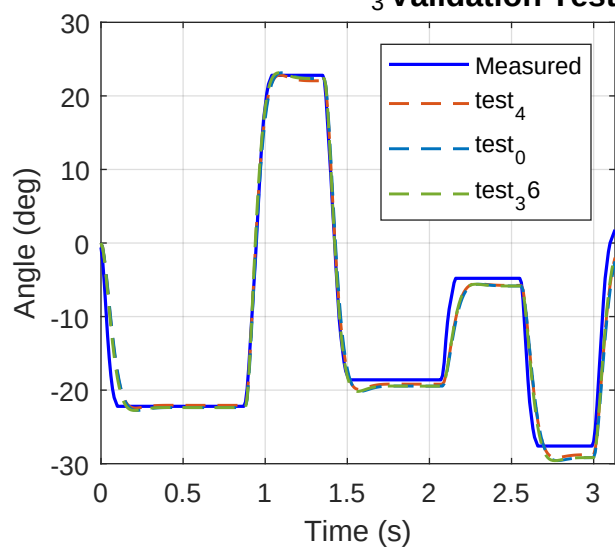
Test 3 Validation Test 0 - model comparison
