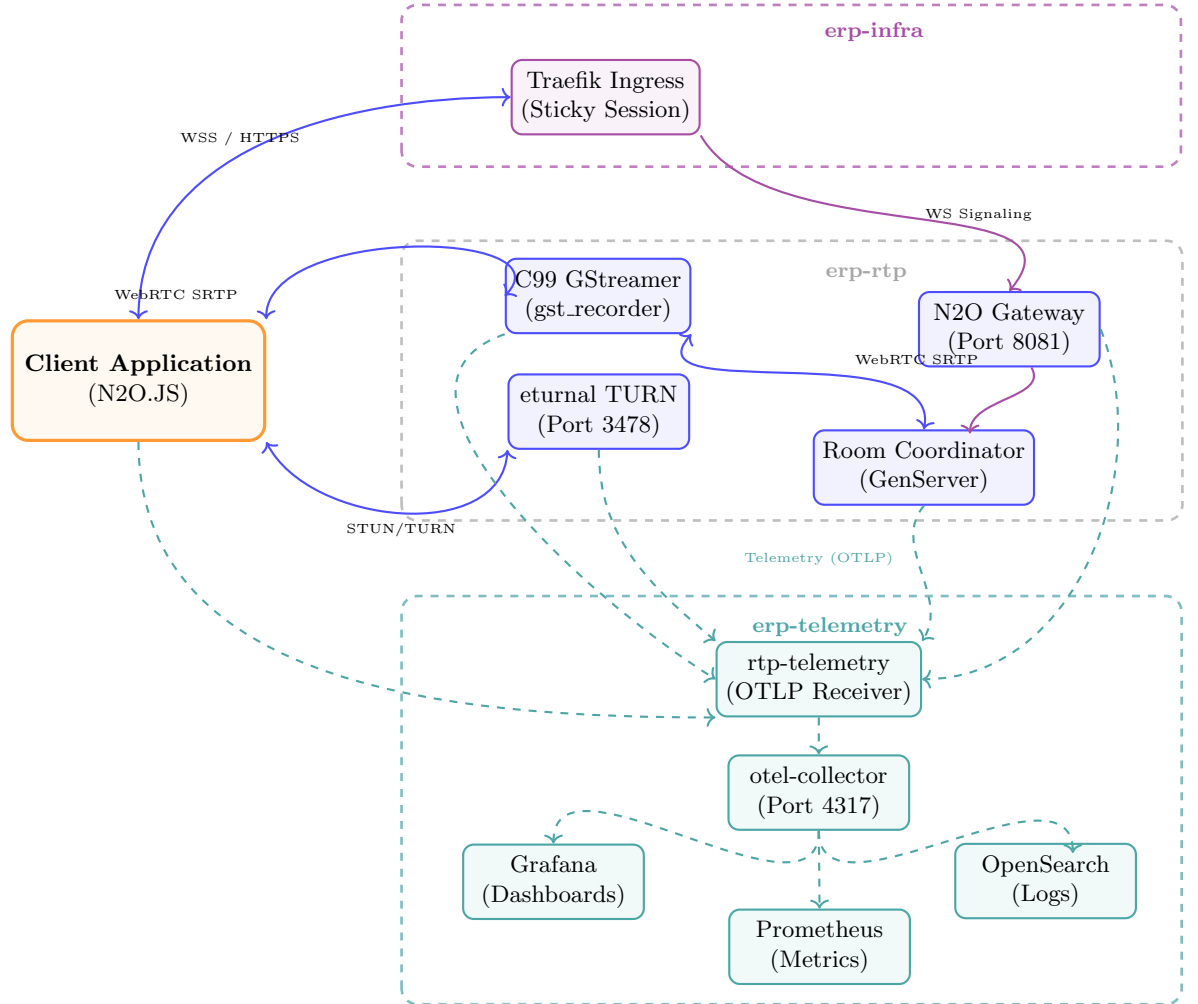
Figure 1: Three-namespaces architecture.
