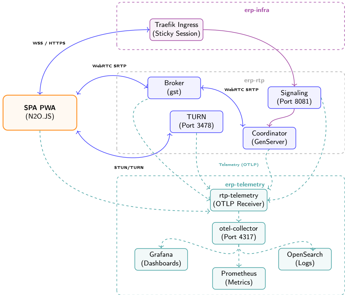
Рис. 1: Three-namespaces architecture.
