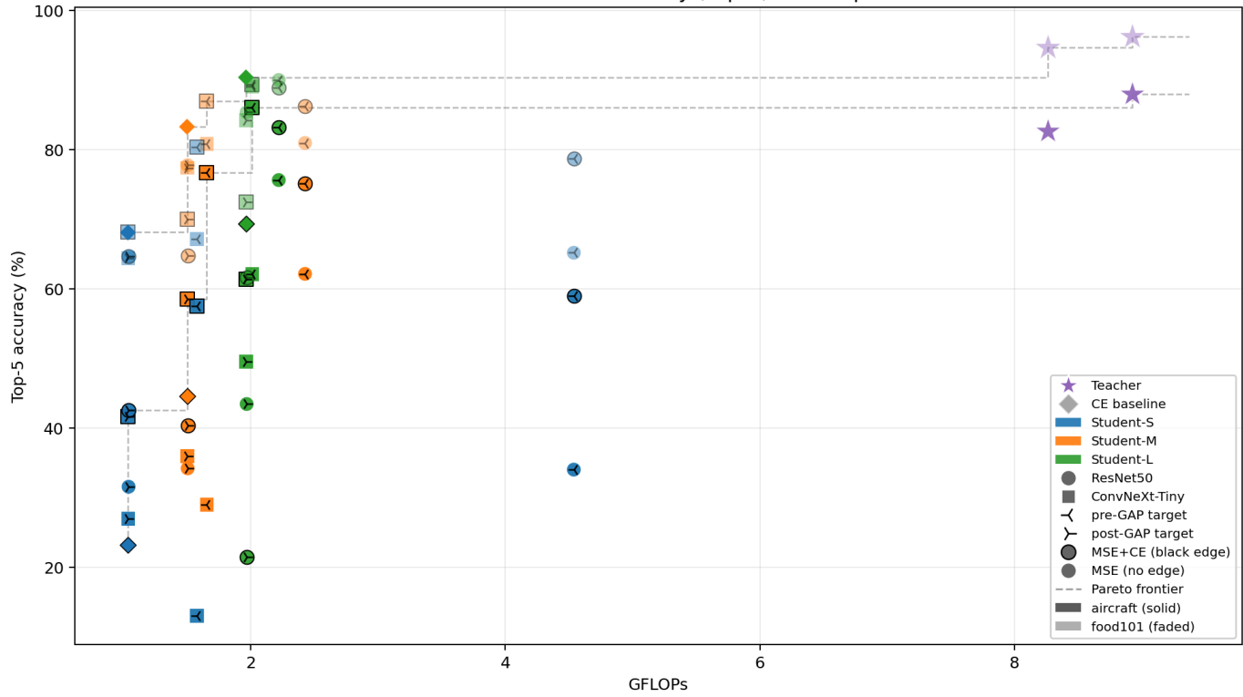
Global overview: Accuracy (Top-5) vs Compute
