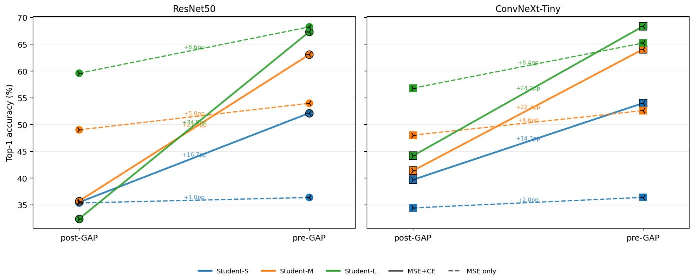
food101: Distillation target comparison — post-GAP vs pre-GAP
