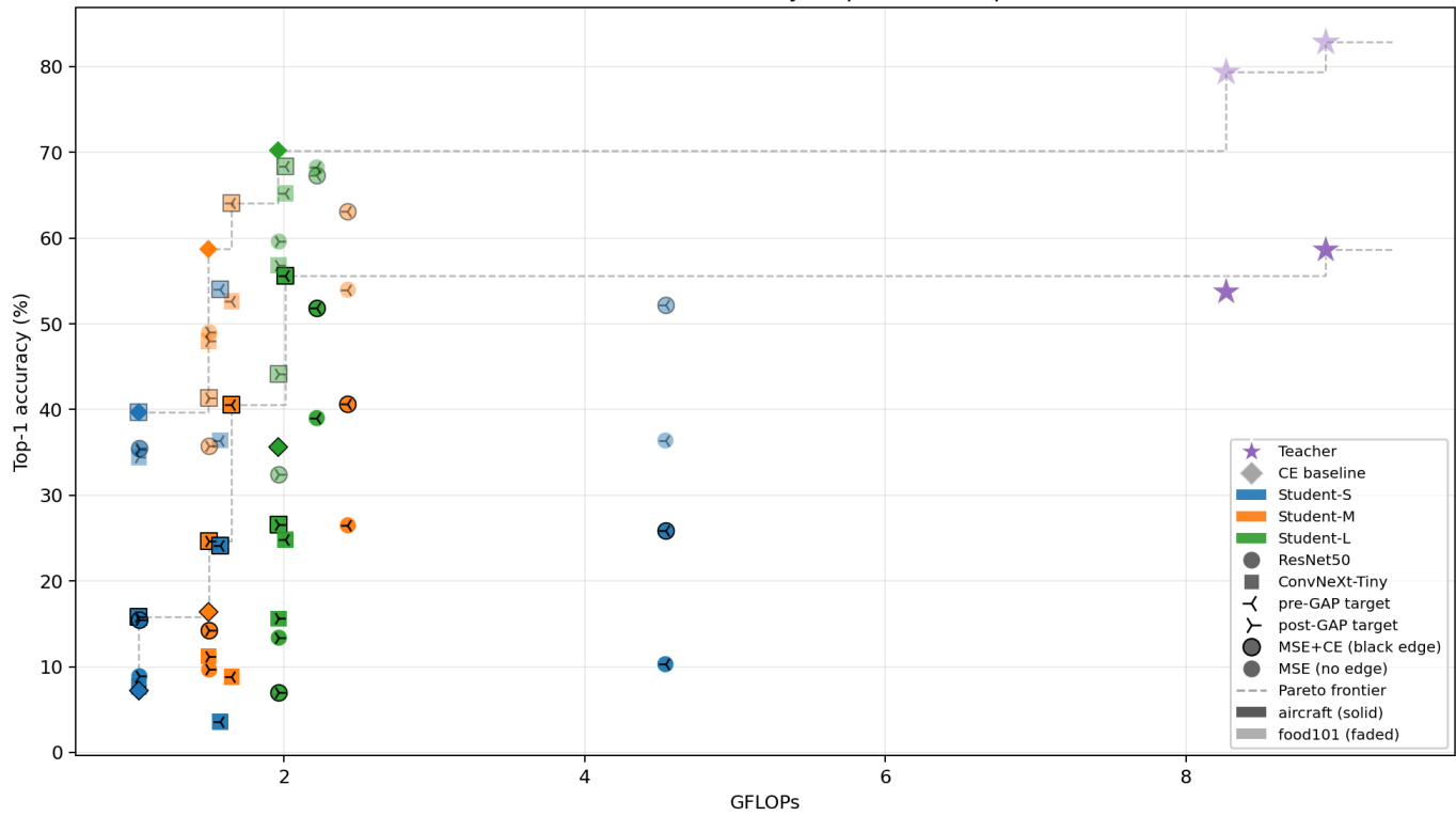
Global overview: Accuracy (Top-1) vs Compute
