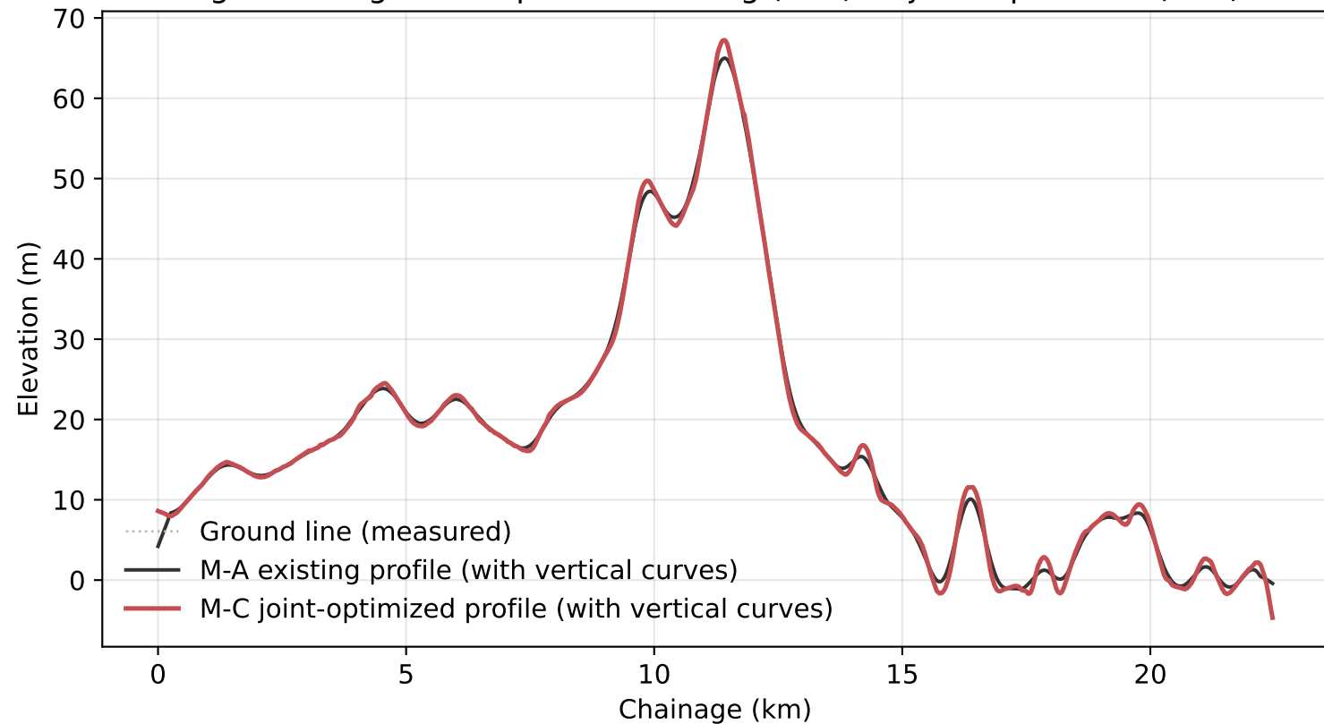
Fig. C3 Longitudinal profile: existing (M-A) vs joint-optimized (M-C)
