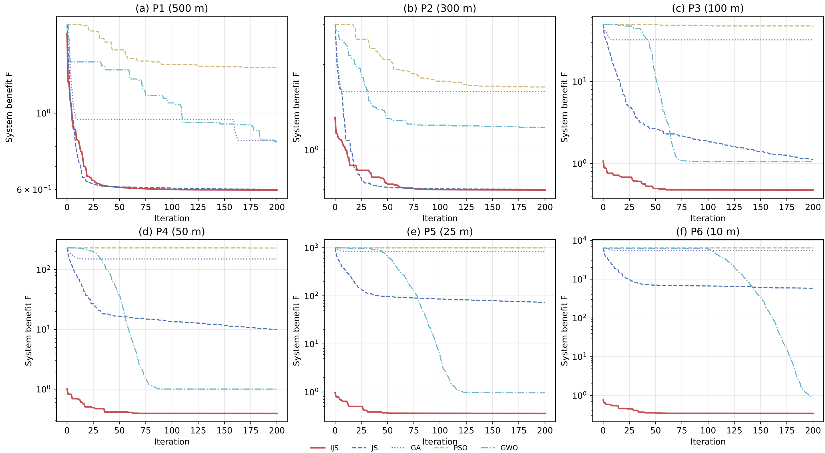
Fig. B1 Convergence curves of algorithms at six problem scales (first 200 generations)
