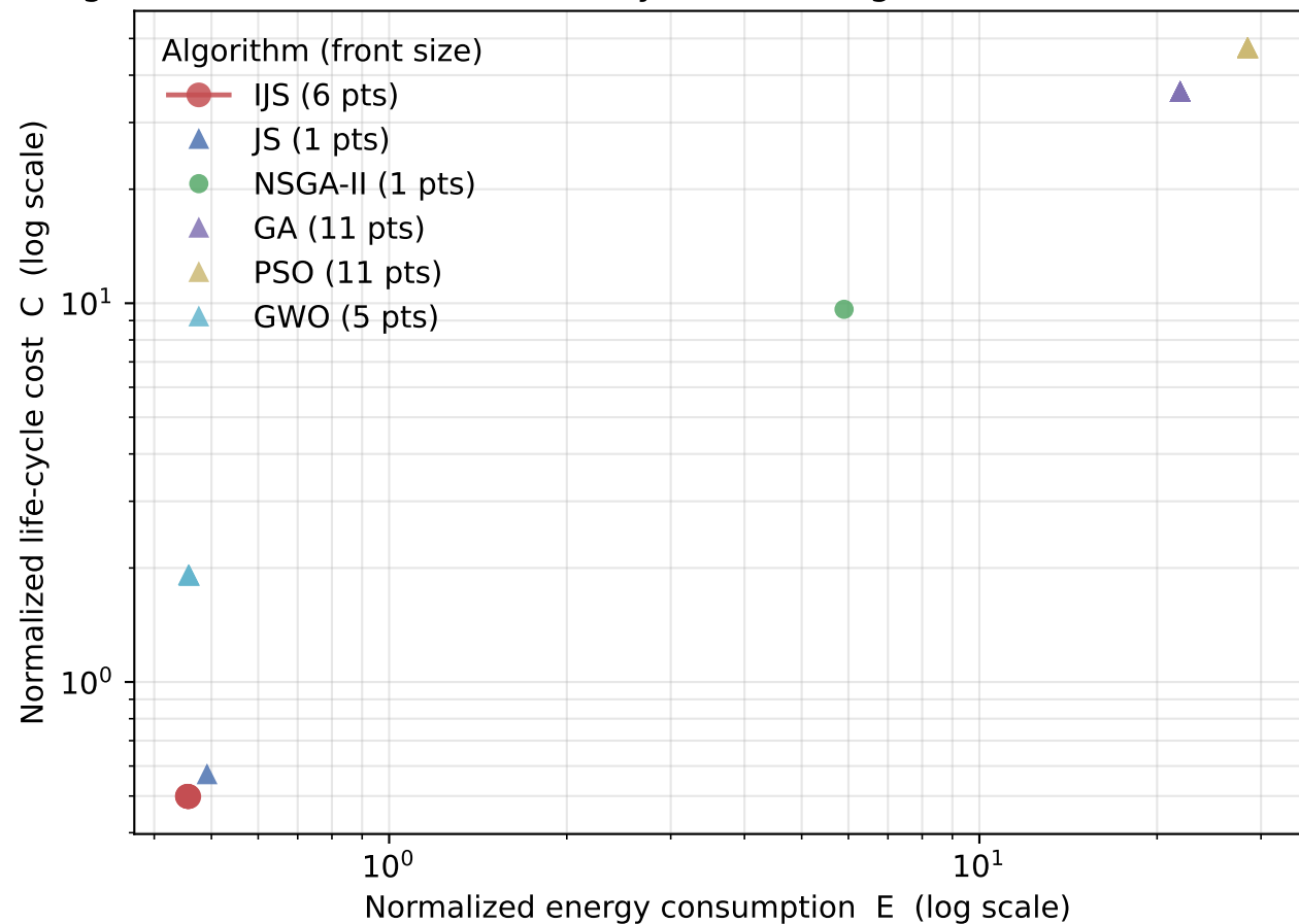
Fig. B2 Pareto fronts obtained by different algorithms (scale P3 (100 m))
