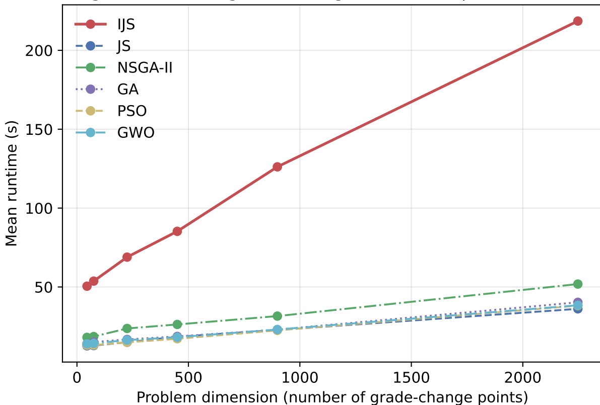
Fig. B3 Runtime growth of algorithms with problem scale
