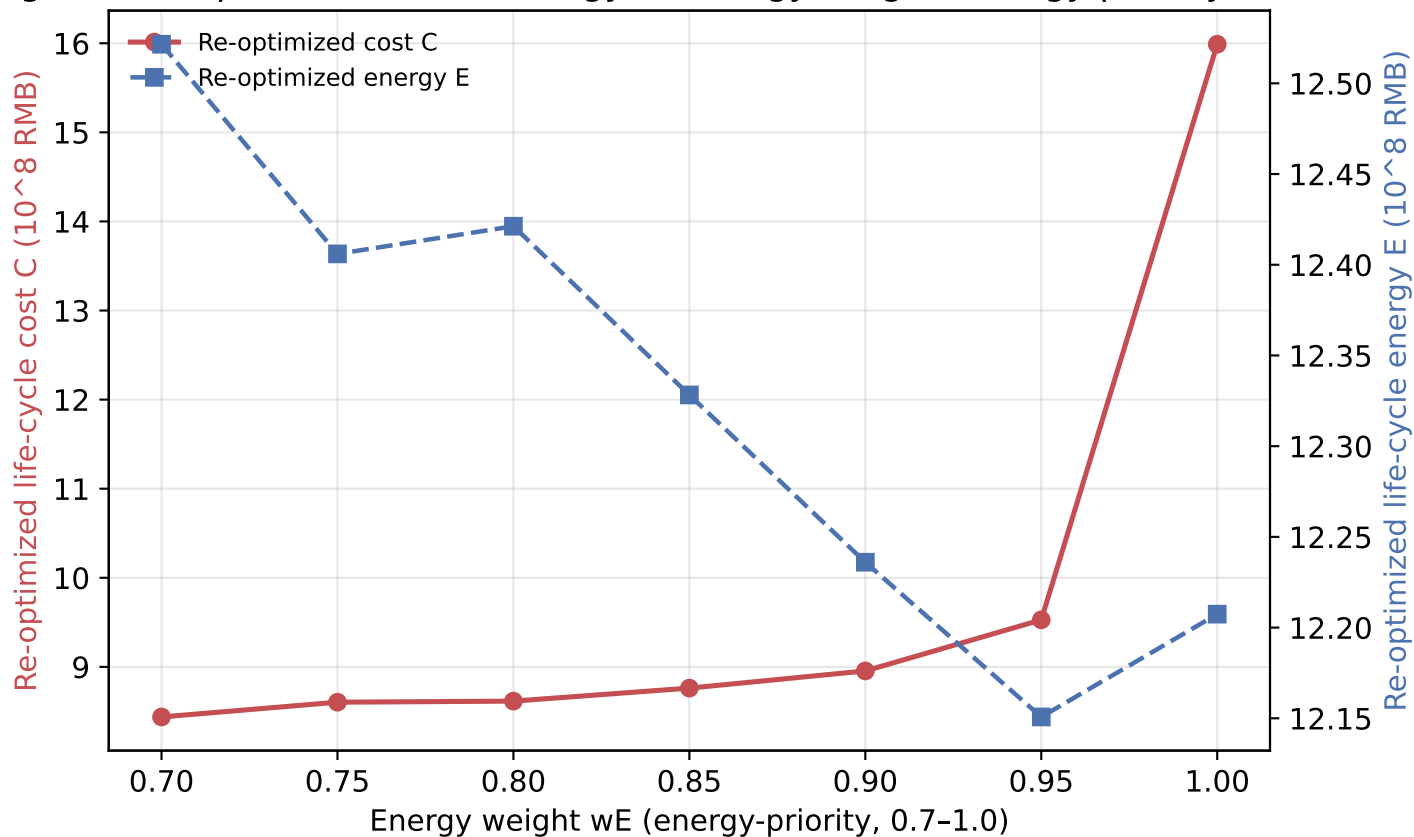
Fig. D7 Re-optimized cost & energy vs energy weight (energy-priority 0.7–1.0)
