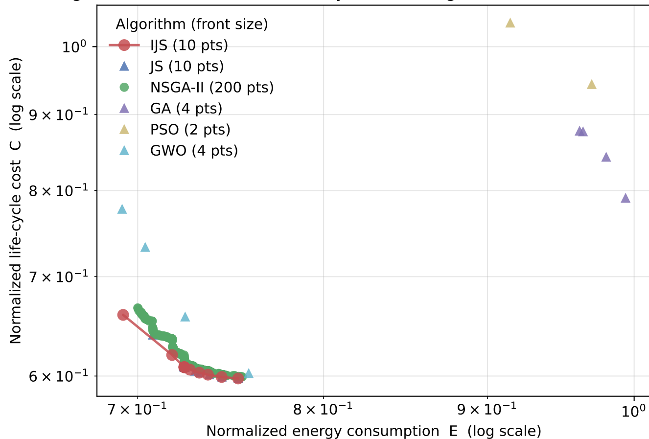
Fig. B2 Pareto fronts obtained by different algorithms (scale P1 (500 m))
