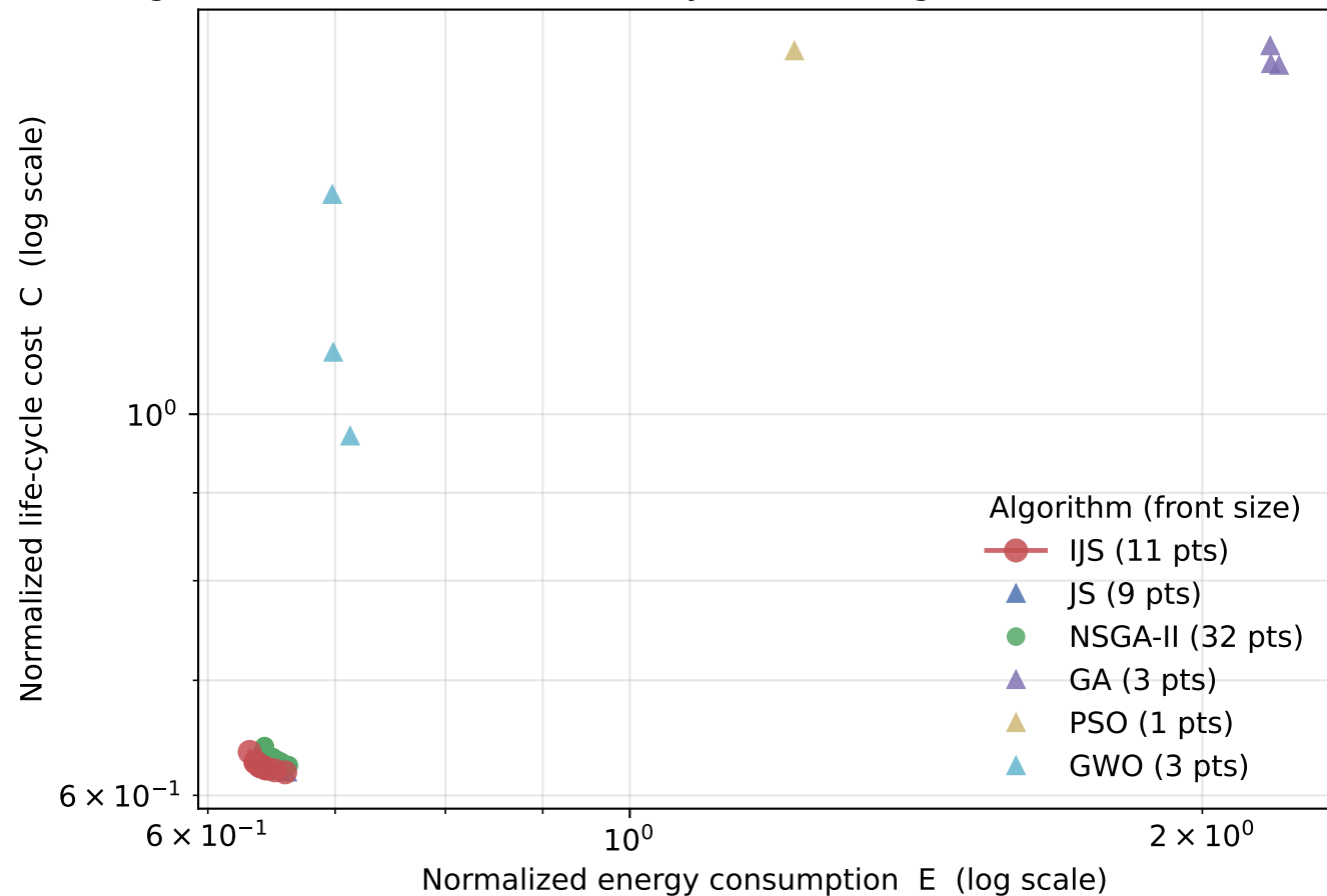
Fig. B2 Pareto fronts obtained by different algorithms (scale P2 (300 m))
