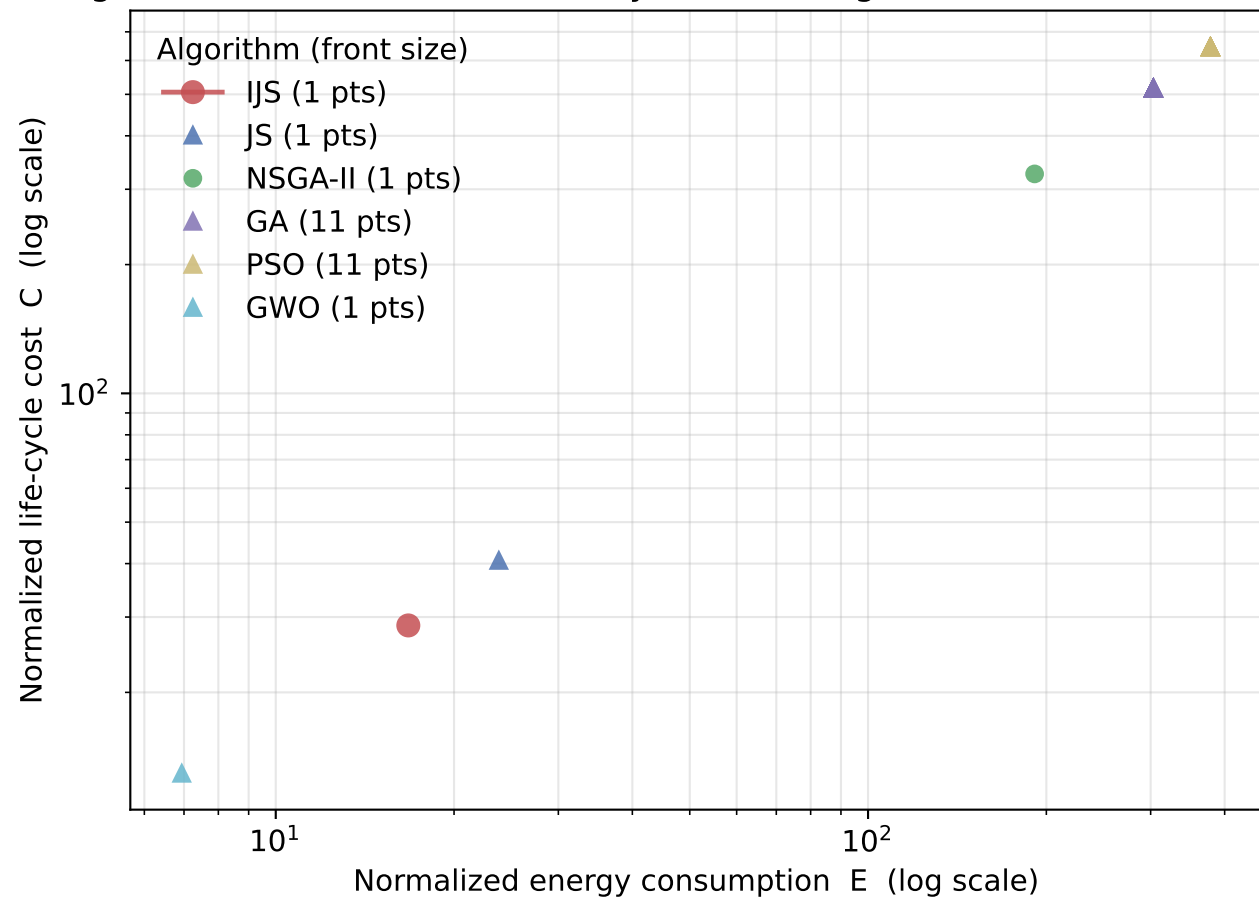
Fig. B2 Pareto fronts obtained by different algorithms (scale P5 (25 m))
