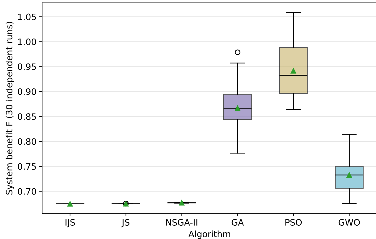
Fig. B4 Box plots of system benefit F across algorithms (scale P1 (500 m))
