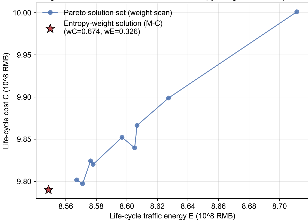
Fig. C1 Pareto solution set and the entropy-weight decision point
