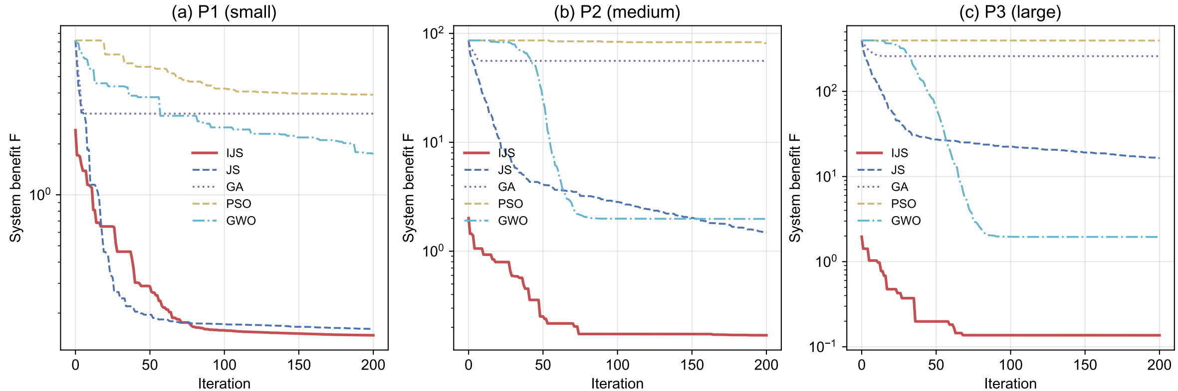
Fig. B1 Convergence curves of algorithms at three problem scales (first 200 generations)
