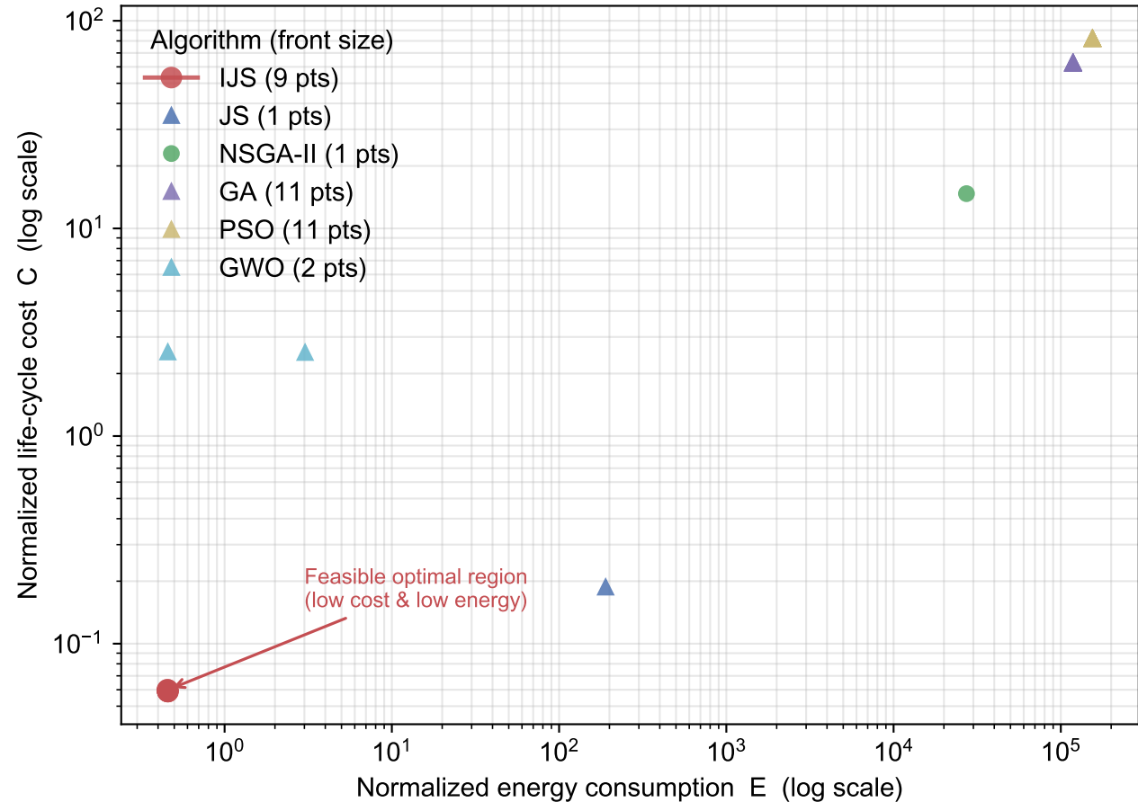
Fig. B2 Pareto fronts obtained by different algorithms (scale P2)
