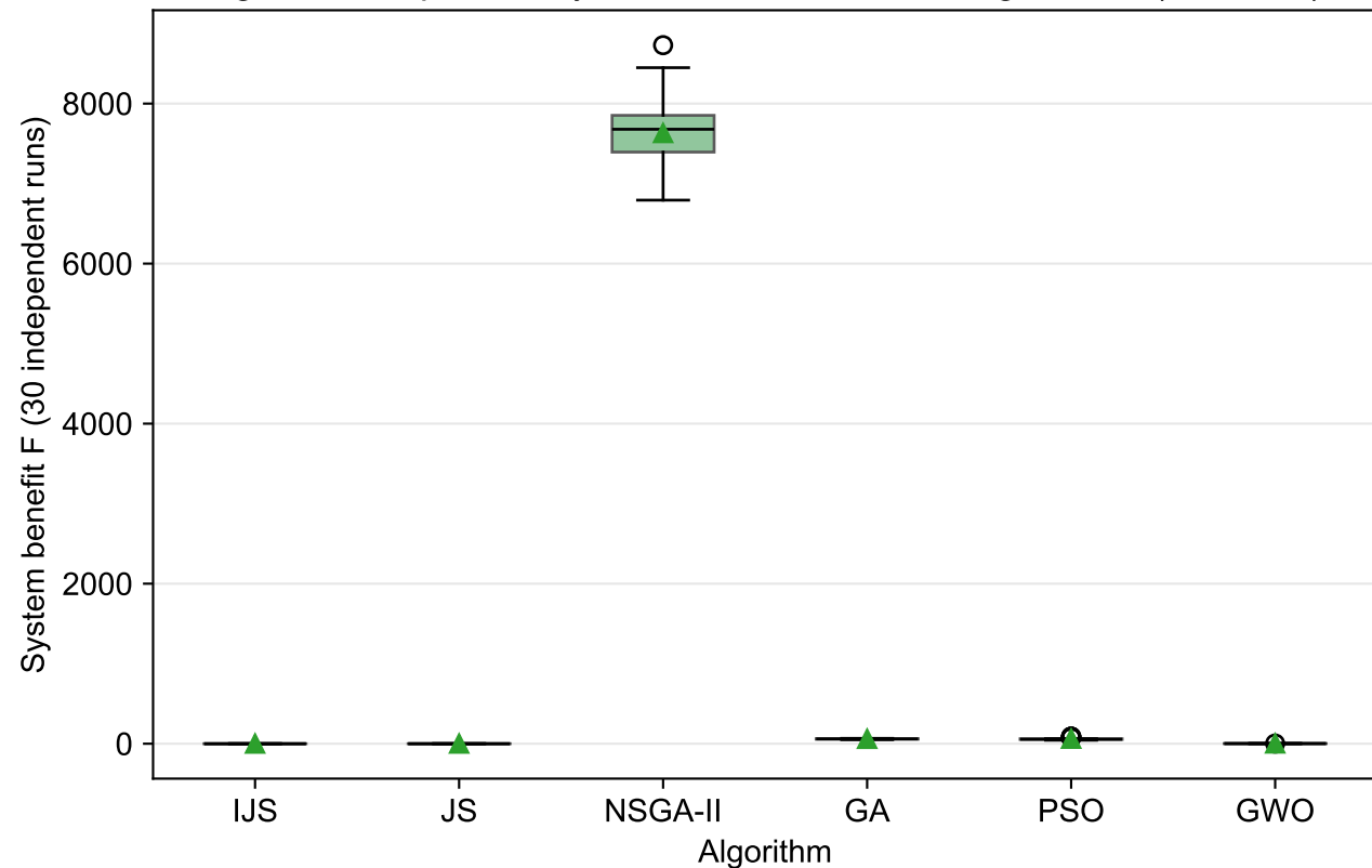
Fig. B4 Box plots of system benefit F across algorithms (scale P2)
