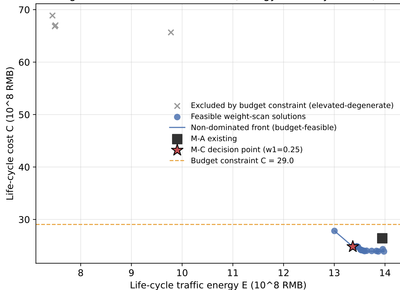
Fig. C8 Full Pareto solution set (energy vs life-cycle cost)
