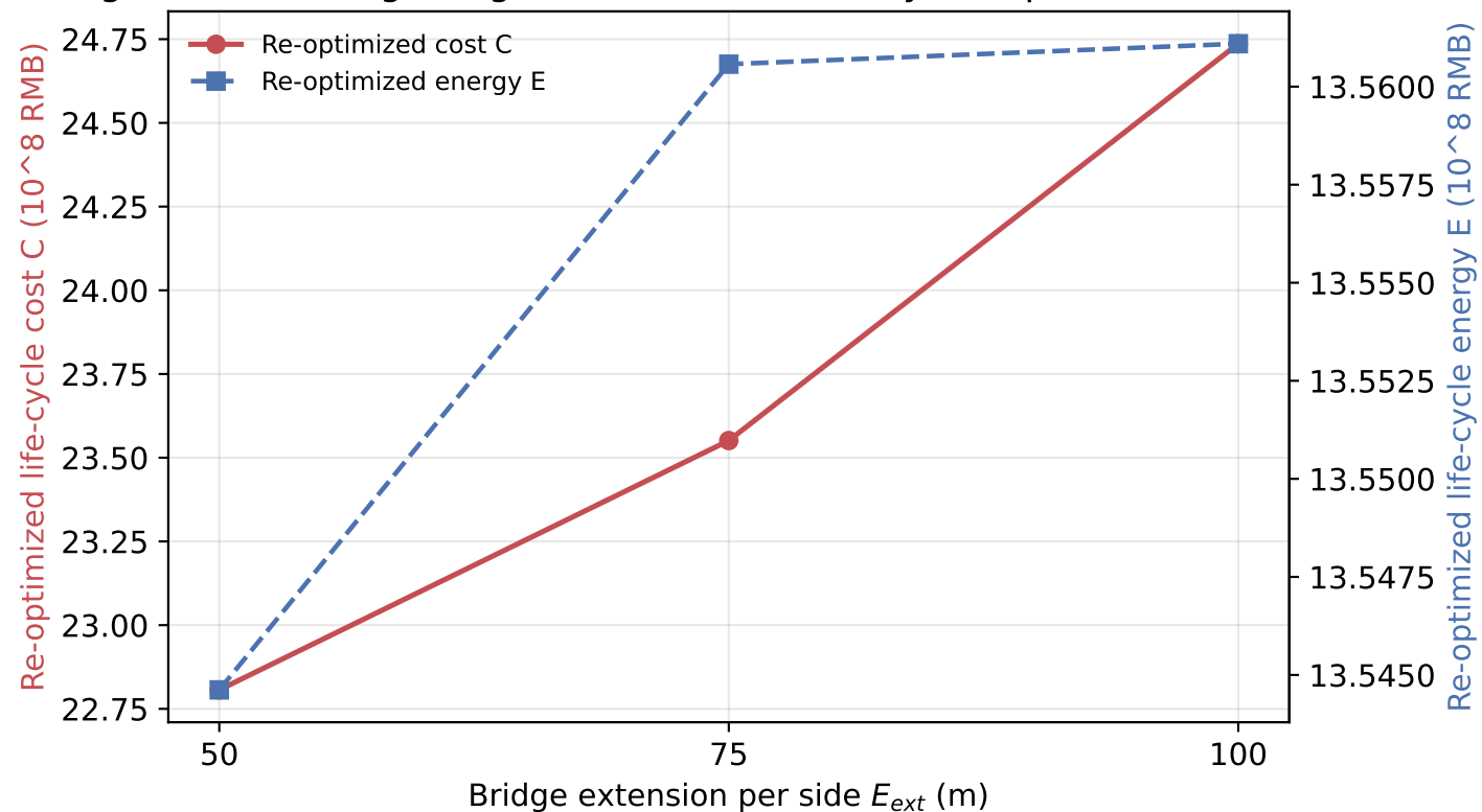
Fig. D10 Crossing-bridge extension sensitivity (re-optimized, w_1=0.65 )
