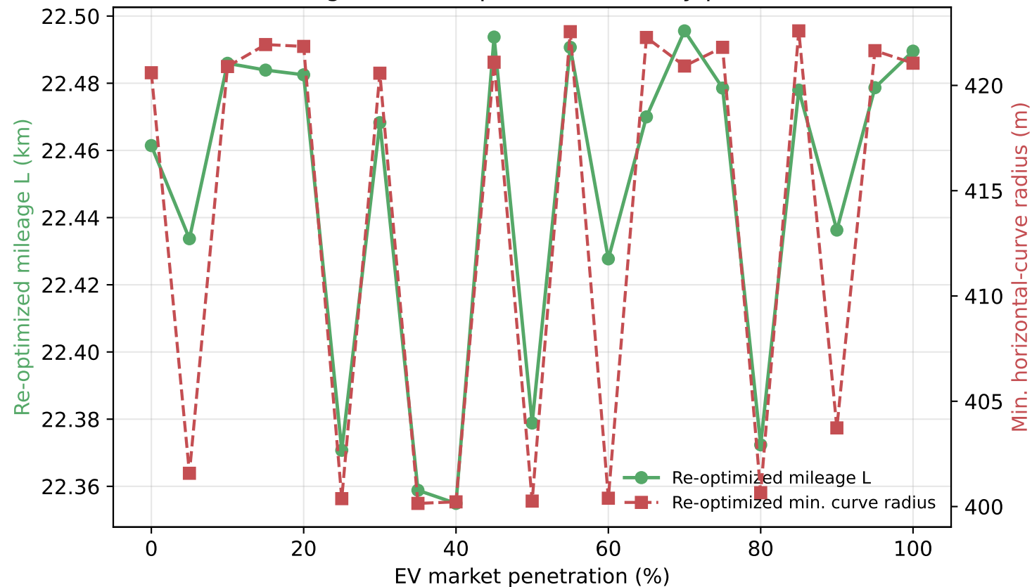
Fig. D5 Re-optimized geometry vs EV penetration (traffic growth 0%) (alignment re-optimized at every point)
