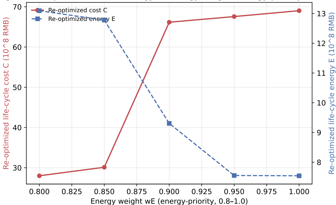
Fig. D7 Re-optimized cost & energy vs energy weight (energy-priority 0.8–1.0)
