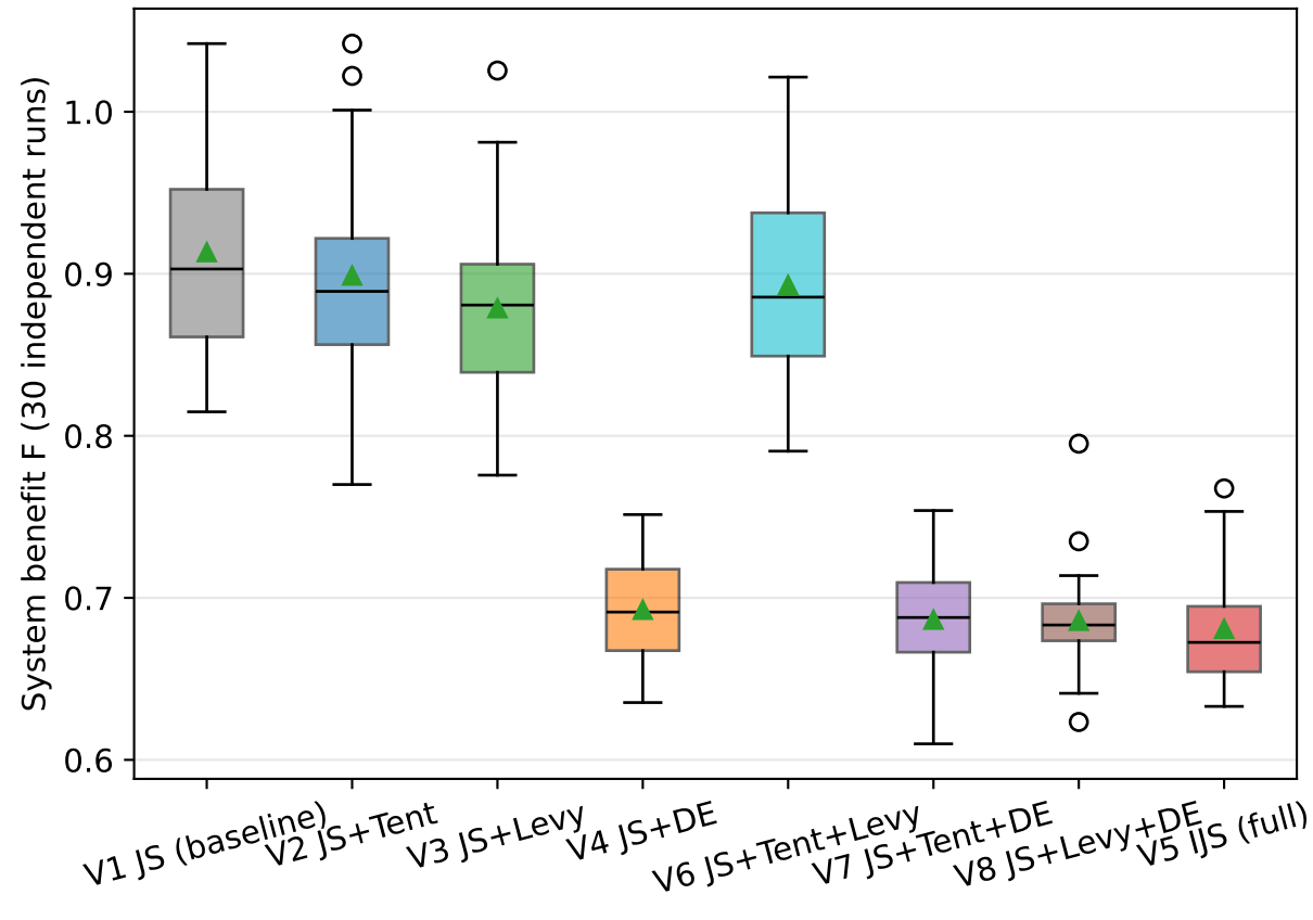
Fig. A3 Box plots of 30 independent runs for each ablation variant
