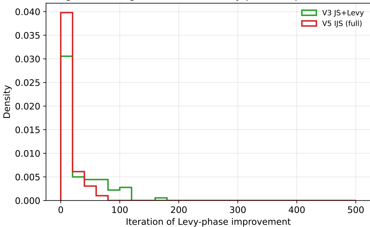
Fig. A6 Timing distribution of Levy-phase improvements
