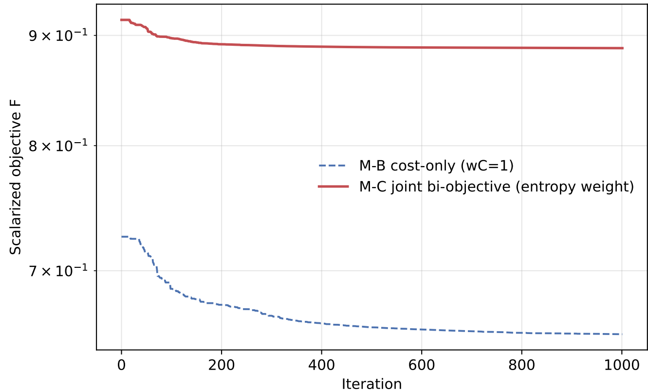
Fig. C6 Convergence of joint plane+profile optimization (IJS)
