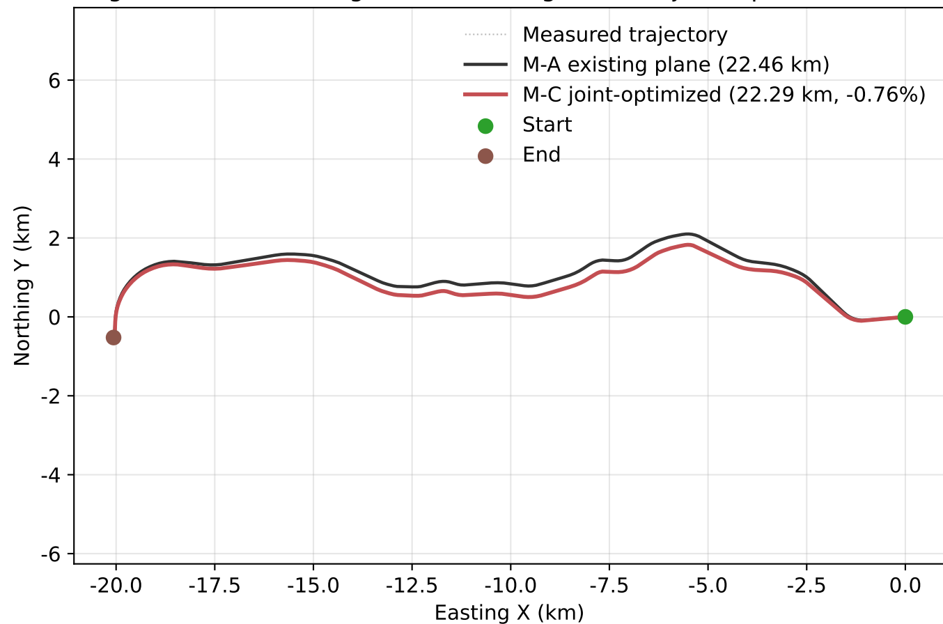
Fig. C2 Horizontal alignment: existing (M-A) vs joint-optimized (M-C)
