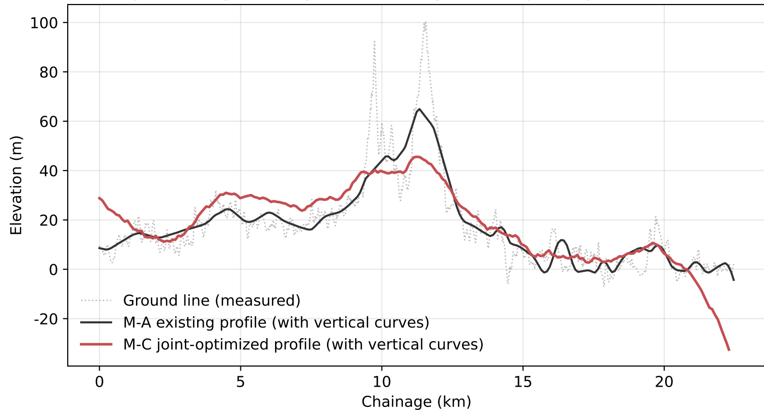
Fig. C3 Longitudinal profile: existing (M-A) vs joint-optimized (M-C)
