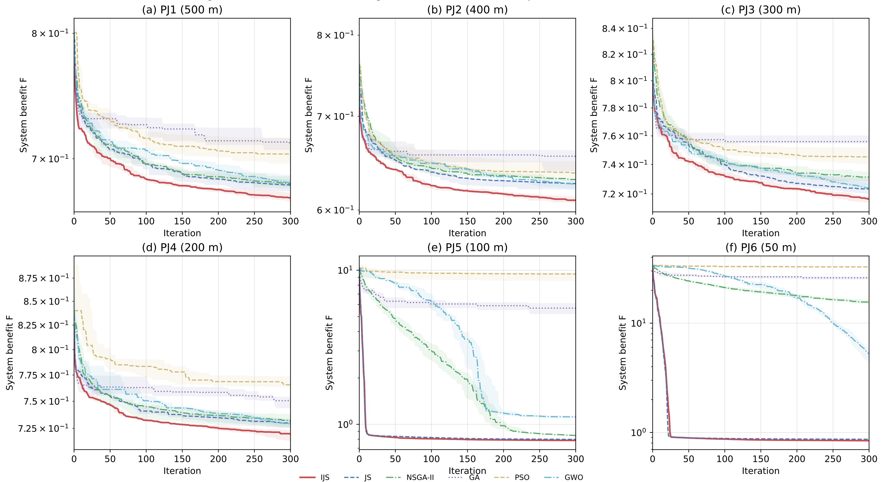
Fig. B1 Pointwise median convergence with IQR over 10 independent runs (300 iterations)
