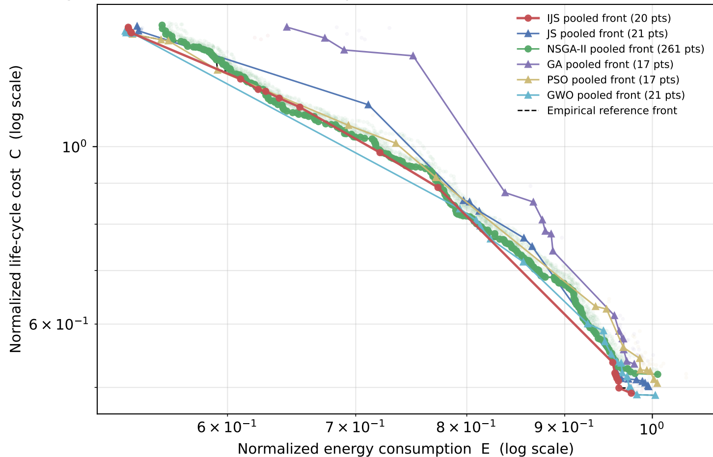
Fig. B2 Pareto fronts over 10 independent runs (300 iterations; scale PJ1 (500 m))
