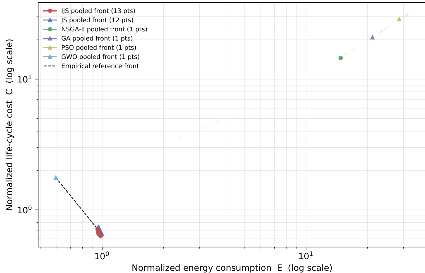
Fig. B2 Pareto fronts over 10 independent runs (300 iterations; scale PJ6 (50 m))
