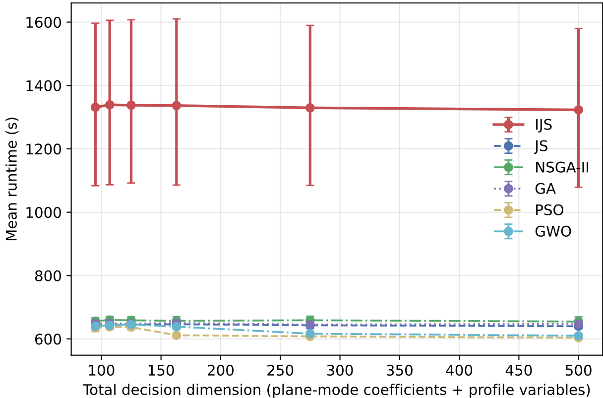
Fig. B3 Runtime versus total decision dimension (mean and 95% CI, 10 independent runs)
