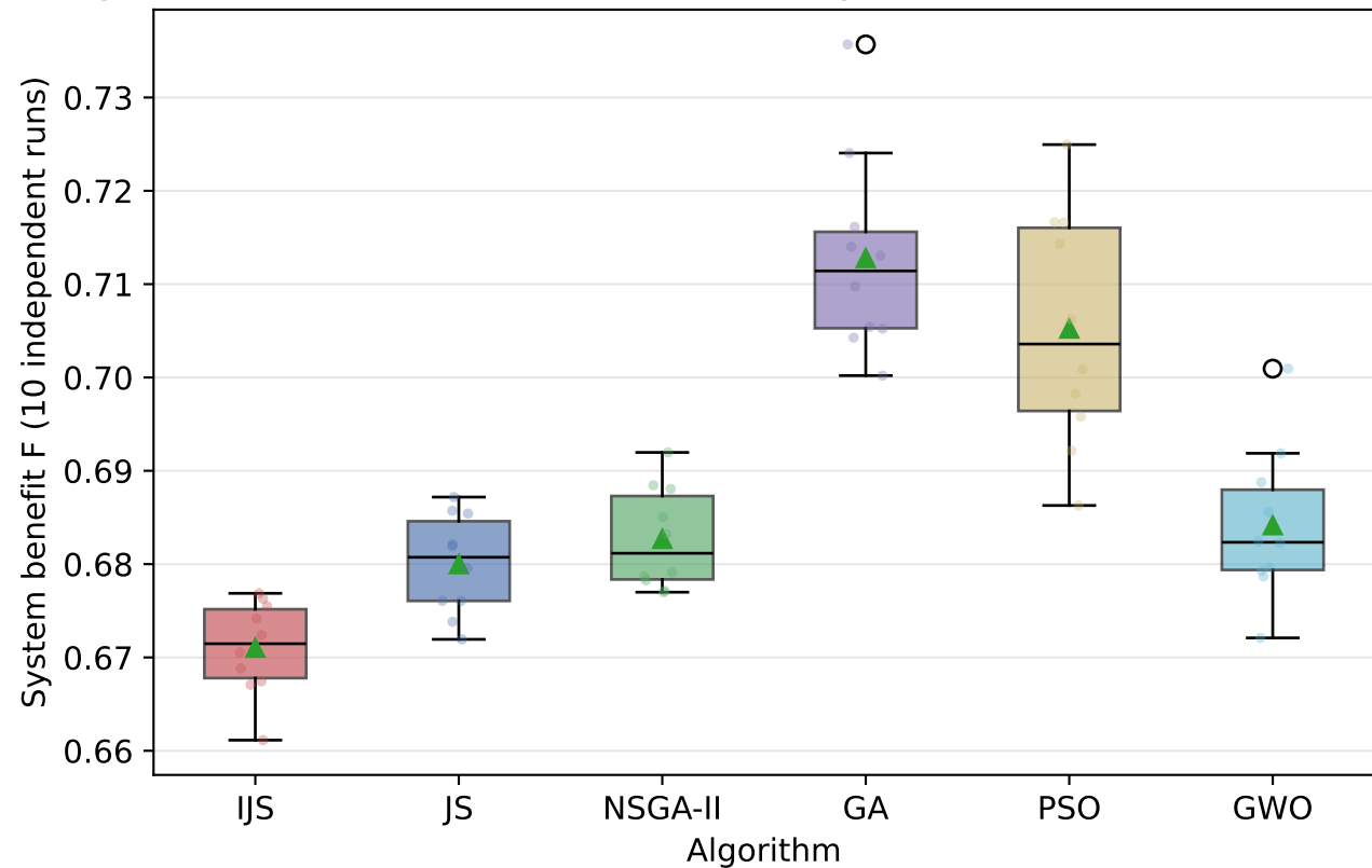
Fig. B4 Final-F distributions over 10 independent runs (scale PJ1 (500 m))
