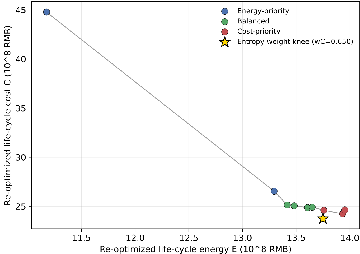
Fig. D4 Cost-energy Pareto front (re-optimized) with weight zones and entropy knee
