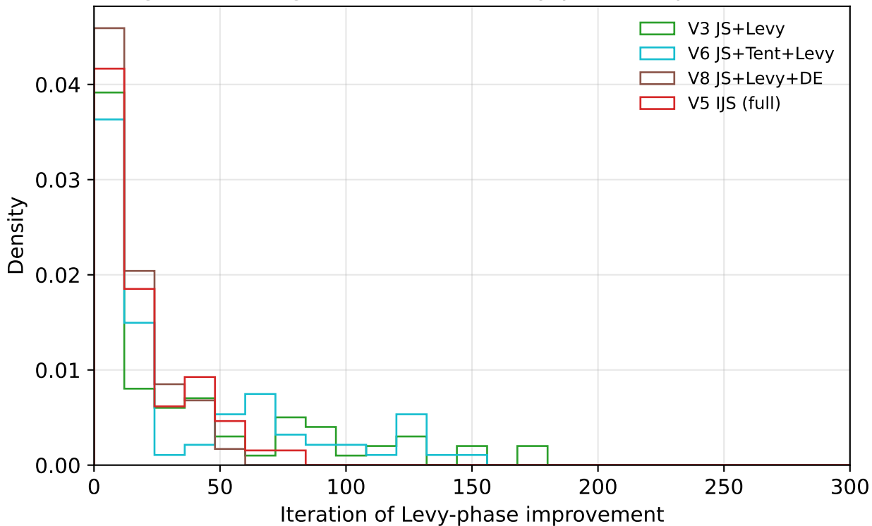
Fig. A6 Timing distribution of Levy-phase improvements
