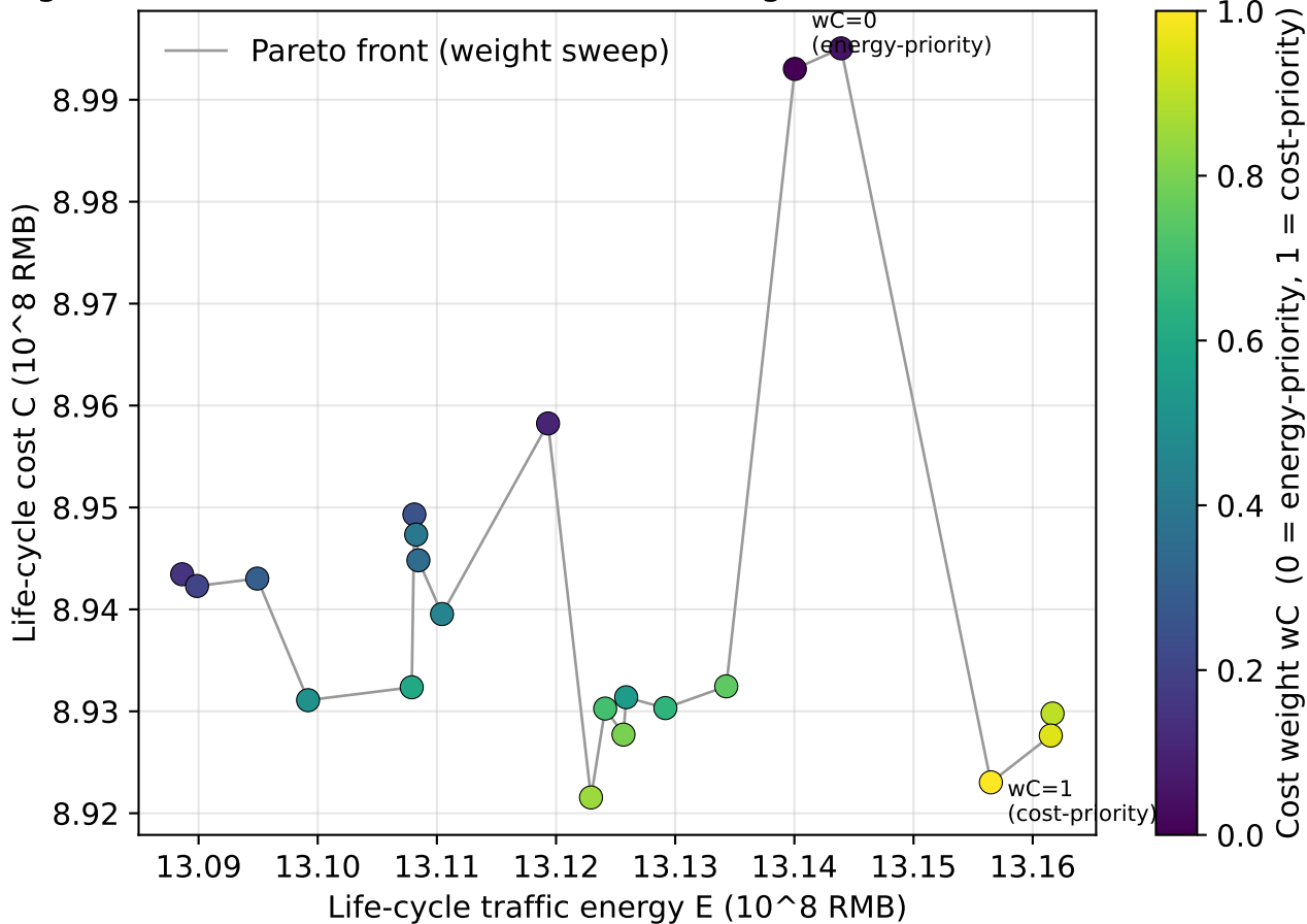
Fig. C7 Pareto front evolution as cost weight w_C varies from 0 to 1
