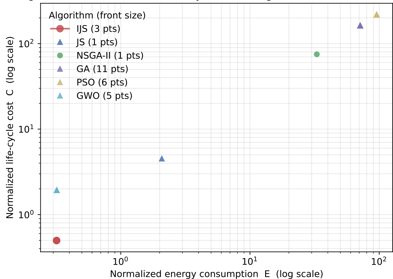
Fig. B2 Pareto fronts obtained by different algorithms (scale P4 (50 m))
