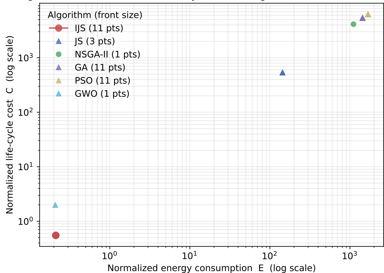
Fig. B2 Pareto fronts obtained by different algorithms (scale P6 (10 m))
