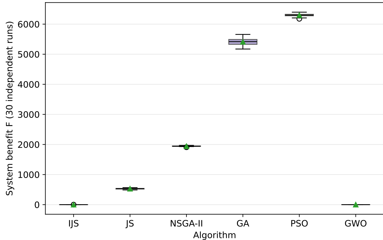
Fig. B4 Box plots of system benefit F across algorithms (scale P6 (10 m))
