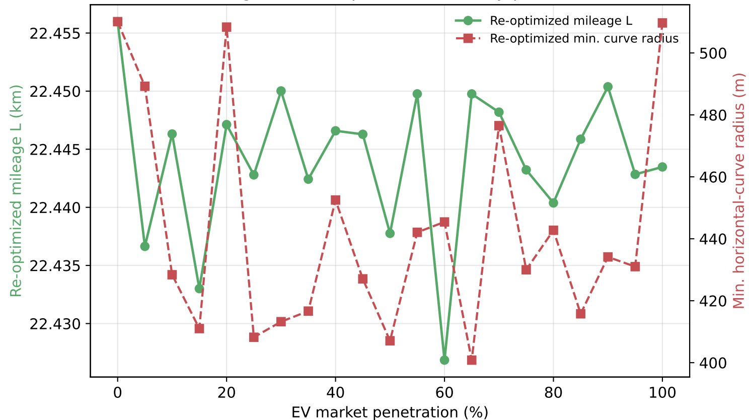
Fig. D5 Re-optimized geometry vs EV penetration (traffic growth 0%) (alignment re-optimized at every point)
